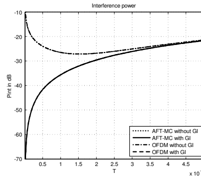
Fig. 7. Comparison of the interference power in the parking scenario for the AFT-MC and OFDM system.
