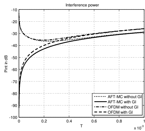
Fig. 10. Comparison of the AFT-MC and OFDM interference power in the LMS channel with LOS component and COST 207 multipath model.
