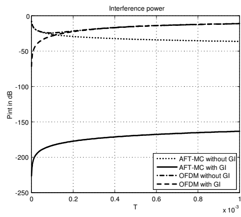
Fig. 8. Comparison of the AFT-MC and OFDM interference power in the two-path LMS channel.
