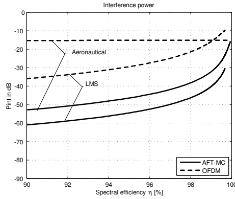
Fig. 3. Comparison of the interference power for different spectral efficiency in aeronautical and LMS channels with the LOS and scattered multipath components.
