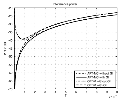
Fig. 5. Comparison of the interference power in the arrival and takeoff scenario for the AFT-MC and OFDM system.
