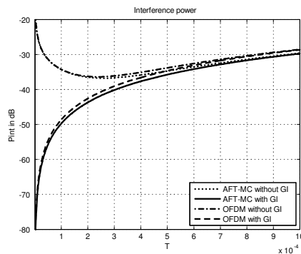
Fig. 6. Comparison of the interference power in the taxi scenario for the AFT-MC and OFDM system.
