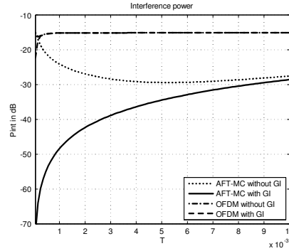
Fig. 4. Comparison of the interference power in the en-route scenario for the AFT-MC and OFDM system.
