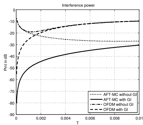
Fig. 9. Comparison of the AFT-MC and OFDM interference power in the LMS channel with LOS component and cluster of scattered paths.
