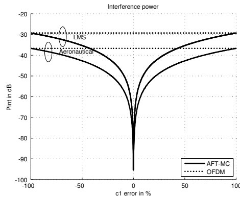
Fig. 2. Comparison of the effects of c_1 estimation errors on the interference power in the AFT-MC and OFDM system in aeronautical and LMS channels.
