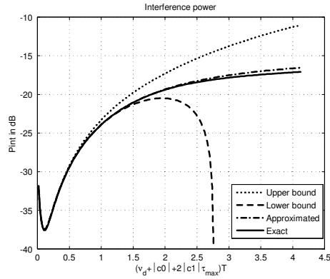
Fig. 1. Comparison of the upper and lower bound, approximated and exact interference power for the AFT-MC system without the GI.
